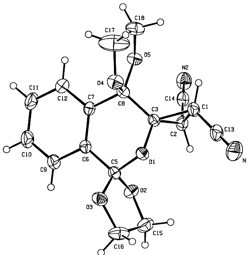
Figure 1. Structure of one molecule of rac - 15 in the crystal; [21] the structure of the other one does not significantly deviate from this; selected bond lengths [Å] and angles [°]: O1–C3 1.392(2), O1–C5 1.444(2), O2–C5 1.383(2), O3–C5 1.384(2), C1–C2 1.519(2), C2–C3 1.505(2), C3–C8 1.506(2), C5–C6 1.502(2), C6–C7 1.388(2), C6–C9 1.389(2), C7–C8 1.511(2), C7–C12 1.391(2), C9–C10 1.367(3), C10–C11 1.383(3), C11–C12 1.368(3); C3–O1–C5 113.33(12), O1–C5–C6 111.53(14), C5–C6–C7 122.21(14), C6–C7–C8 120.20(14), C3–C8–C7 107.92(14), O1–C3–C8 111.81(12), C1–C3–C2 60.76(11)
